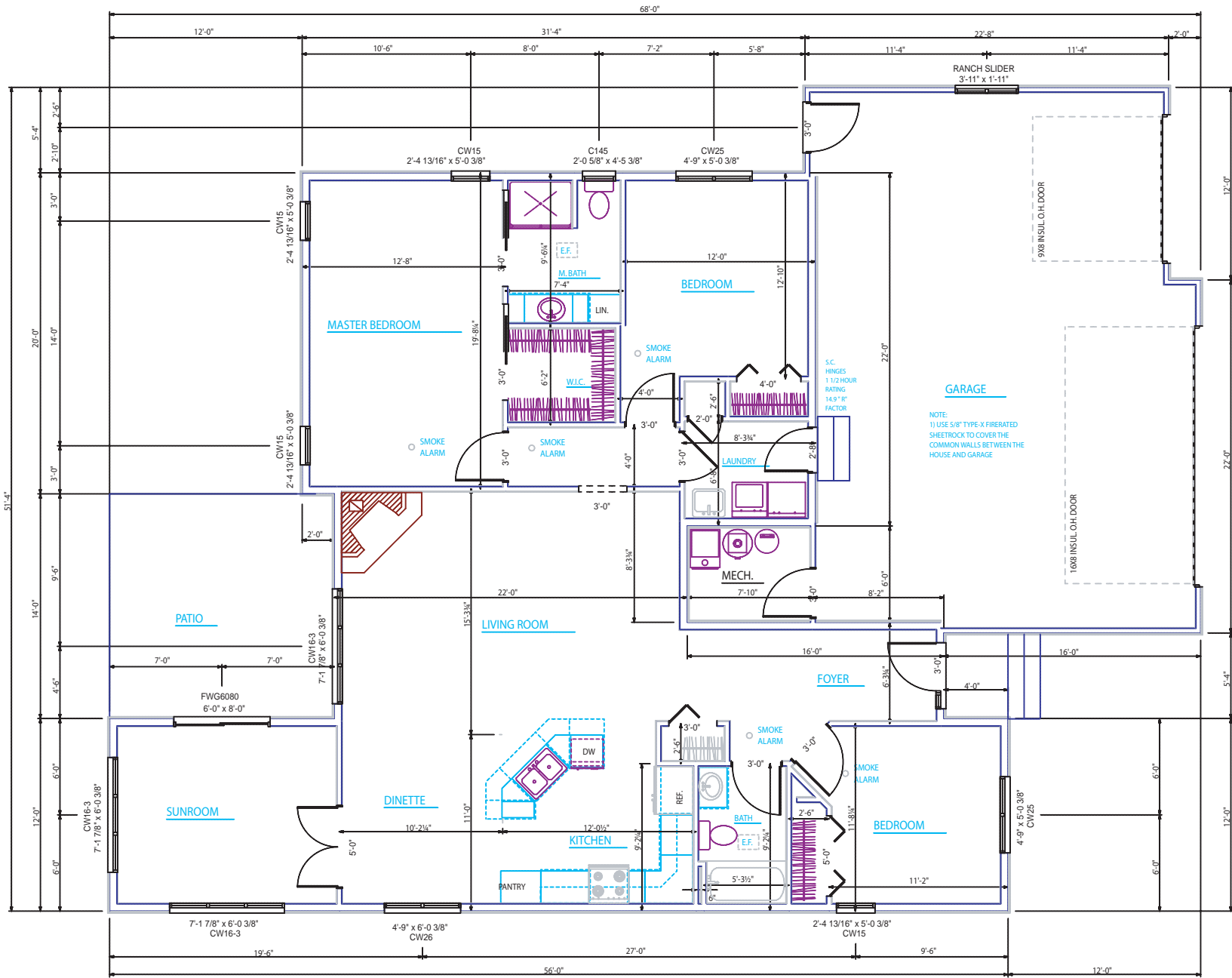
MAIN FLOOR PLAN SCALE: 1/4" = 1'-0" 1750 SFT.
